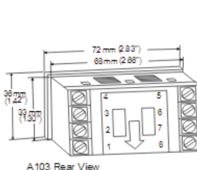
Option Module Rear View
